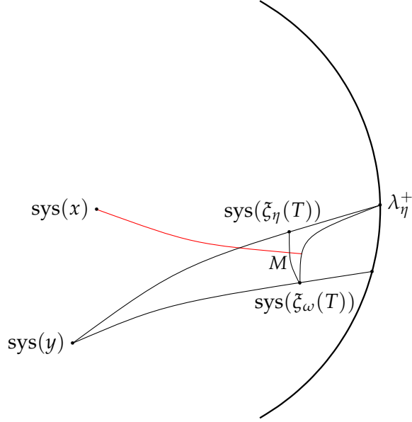
FIGURE 2. The Gromov product (\text{sys}(\xi_\omega(T)), \lambda_\eta^+)_{\text{sys}(x)} in \mathcal{C}(S) , up to an additive constant.
