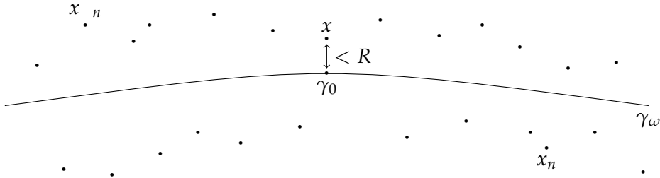
FIGURE 1. A sample path \omega in \Lambda_R .
