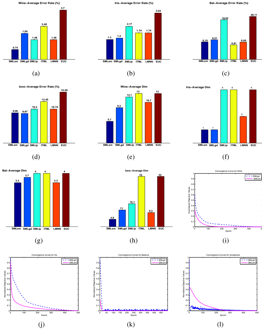
Figure 1: Performance comparison among different methods. Subfigures (a)-(d) present the average error rates; (e)-(h) plots the average dimensionality used in different methods; (i)-(l) give the convergence graph for the sub-gradient algorithm and the proposed smooth optimization algorithm.
