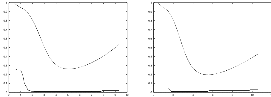
Figure 3: Generalisation error (solid curve) and upper bound from VC theory (dashed curve with R=1 ) for digits 0 and 3 from the USPS dataset of handwritten digits.
