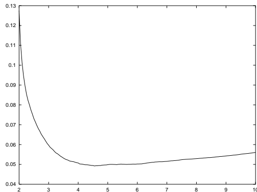
Figure 1: Generalization error ( y -axis) as a function of \sigma ( x -axis) for the mirror symmetry problem (for Gaussian kernels with zero training error and maximal margin, m = 200 , n = 30 and averaged over 10^5 examples).
