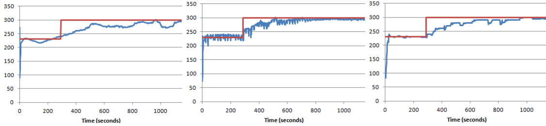
Figure 5: Illustrative example of a positive market shock, from P_0^t = 230 to P_0^{t+1} = 300 . Markets containing only ZIP_M agents (centre) re-equilibrate after a market shock more quickly than ZIP_S (left) and AA_D (right). Results for negative market shocks ( P_0 falls) are symmetrically similar.
