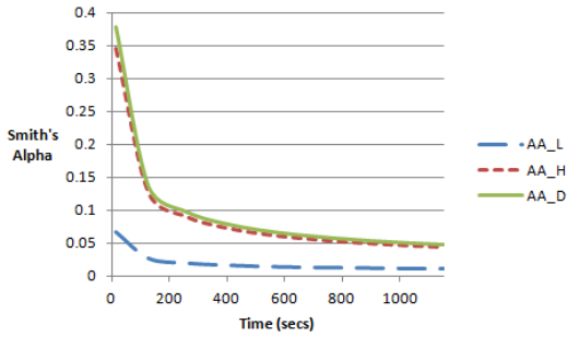
Figure 3: Smith’s \alpha over time for each homogeneous AA market. AA_L produces lower alpha than AA_H , demonstrating that lower values of P_{max} artificially encourage equilibration.
