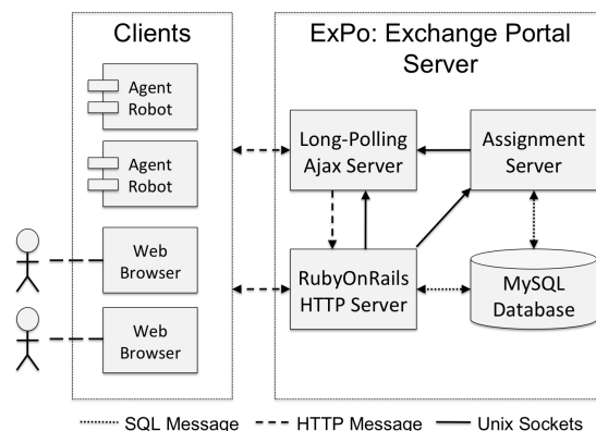
Figure 1: ExPo Architecture. The ExPo exchange is a Ruby on Rails web server application with RESTful architecture, using a MySQL database for storage. Clients (automated trader agents, or human traders using a web browser) connect and message the server using HTTP messaging. ExPo internal servers communicate via unix sockets.
