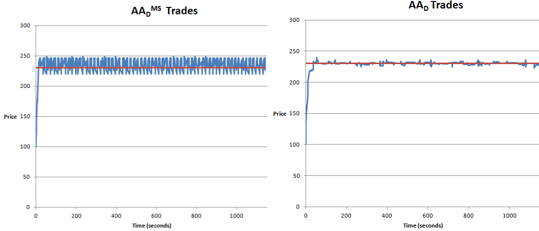
Figure 4: Trades in homogeneous markets. Left: AA_D^{MS} agents ( maxSpread = 15\% ). Right: AA_D agents ( maxSpread = 0\% ).
